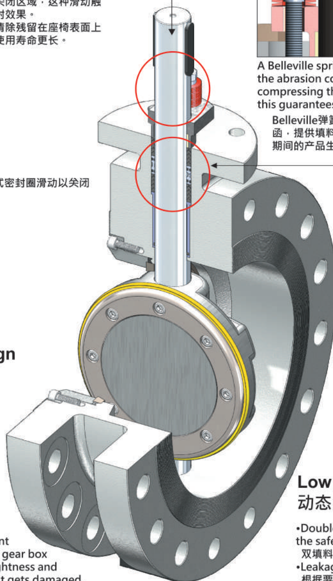
Disc seal ring seated 刮刀密封圈座
