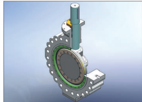
SolidWorks 3D SolidWorks 3D 设计
