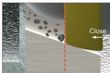
Disc seal ring sliding to close 刮刀式密封圈滑动以关闭
