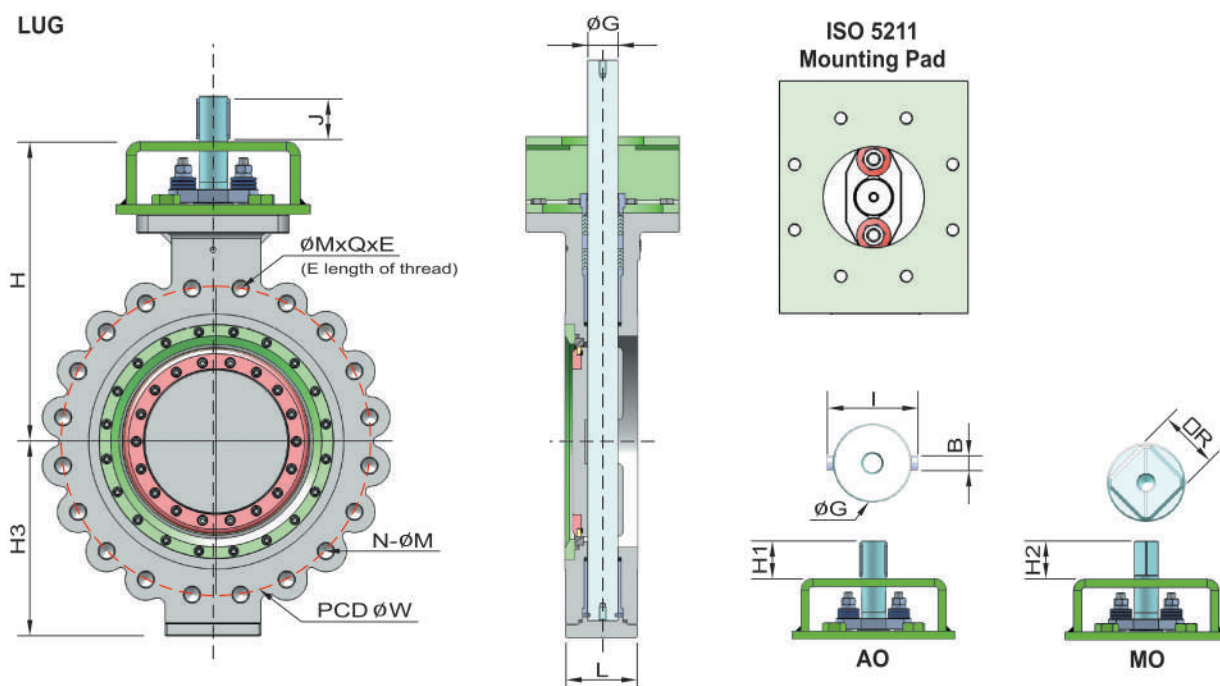
DIMENSIONS (ASME CLASS 150 LUG) 尺寸 (mm)
