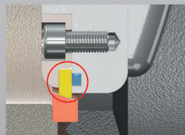
After seat contact 密封后
