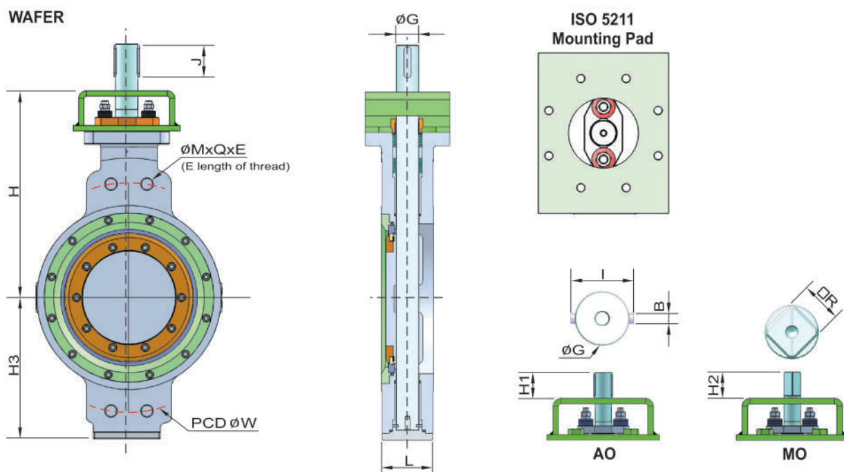
DIMENSIONS (ASME CLASS 150 WAFER) 尺寸
